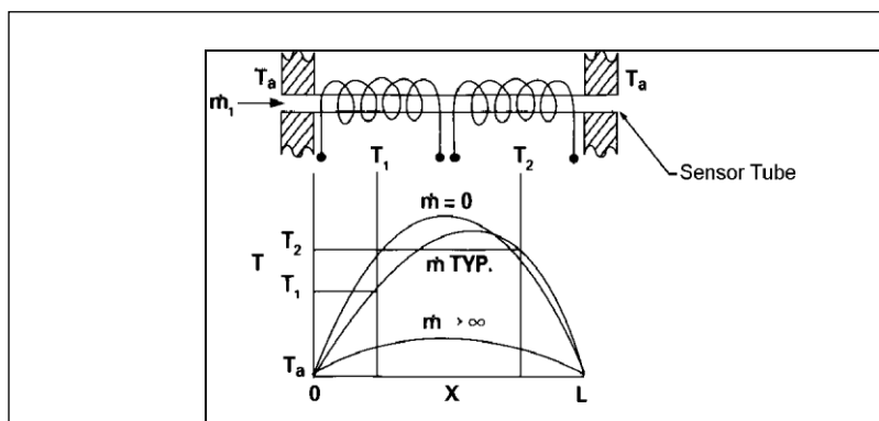
Figure 1-4. Sensor Temperature Distribution
